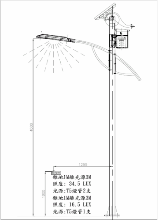
A. 16.5 Lux at 1 meter height from ground level.
